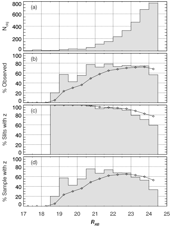
FIG. 7.— Completeness indicators as a function of R_{AB} magnitude in the TKRS sample. (a) The number of available targets N_{obj} per 0.5 mag bin in our GOODS-N field target catalog, to the limiting magnitude of R \leq 24.4 . (b) Differential fraction of available targets (relative to the total sample available within each 0.5 mag bin) for which spectra were acquired ( shaded histogram ), or the integrated fraction to that magnitude bin ( connected diamonds ). (c) Differential and integrated fraction of spectra which yielded secure redshifts. (d) Differential and integrated fraction of available targets which yielded secure redshifts, including objects not observed.
